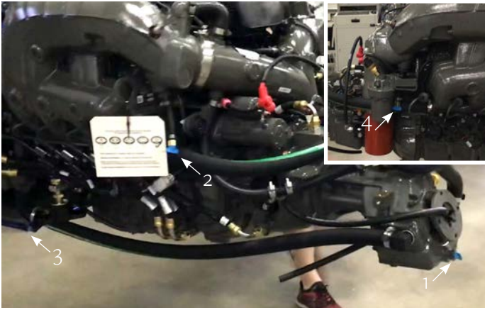
1 - Under the heat exchanger 2 - The bank 1 manifold. 3 - The V-drive 4 - The bank 2 manifold.
